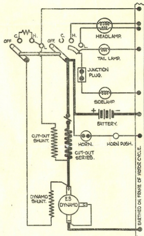
TECHNICAL WIRING DIAGRAM
