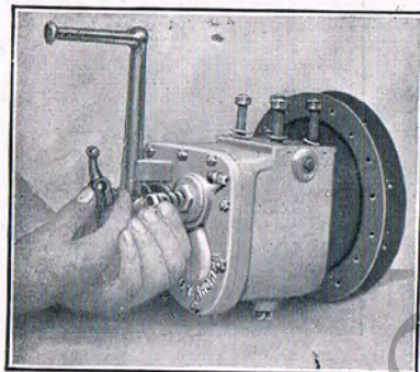
Taking off Clutch Control and operating worm.
