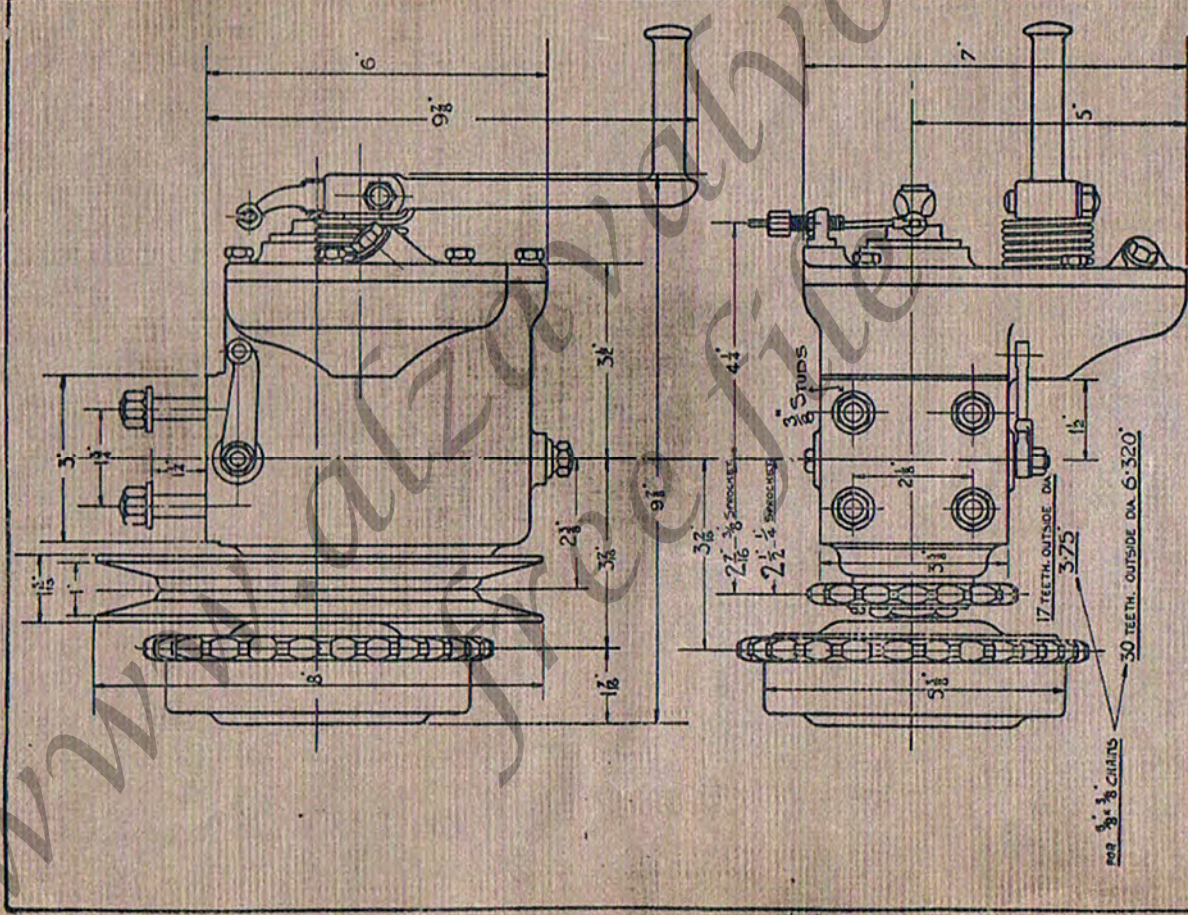
STURMEY-ARCHER 3-SPEED C.S. GEAR GEAR-RATIOS 1:1.632 : 2.662 FLEET PLAN
